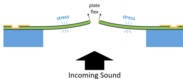
Figure 11: Piezoelectric plate stress in response to sound pressure
