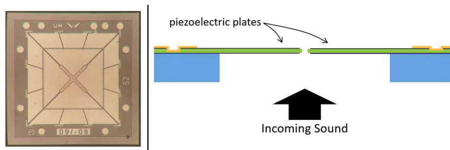
Figure 10: Top-view (left) & cross-sectional drawing (right) of Vesper piezoelectric MEMS microphone, not to scale
