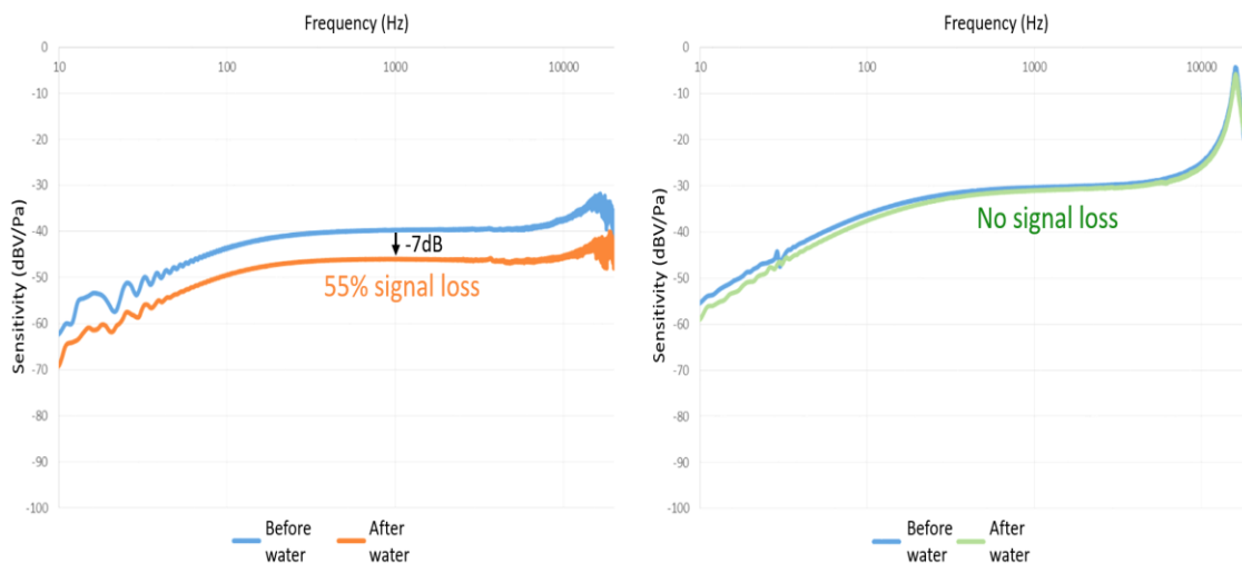
Figure 16: Water-test results of capacitive MEMS microphone (left) and Vesper piezoelectric MEMS microphone (right)
