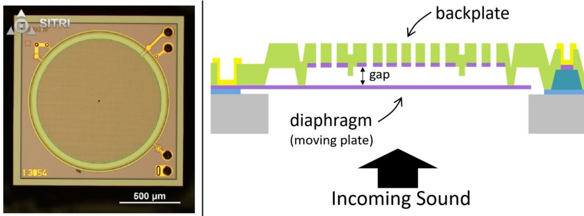
Figure 8: Top-view (left) & cross-sectional drawing (right) of capacitive MEMS microphone
