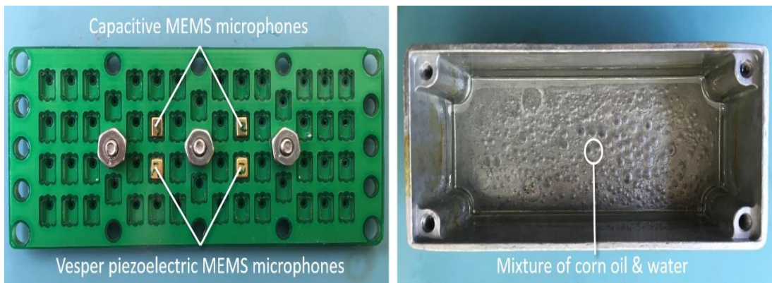
Figure 17: Apparatus for depositing kitchen oil on the surface of microphones, with lid (left) screwed onto an oil chamber (right)
