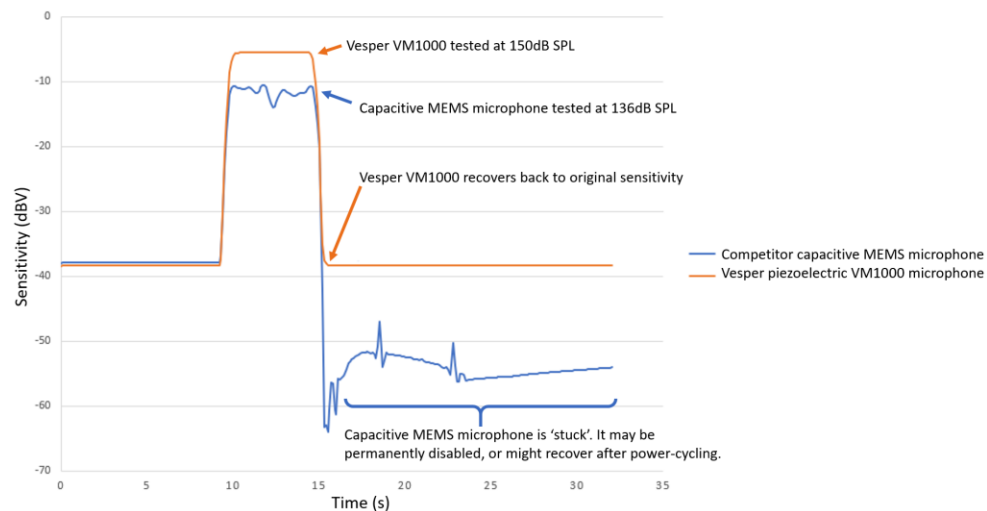
Figure 19: Acoustic Overload test results of capacitive MEMS microphones (blue line) and Vesper piezoelectric MEMS microphones (orange line)
