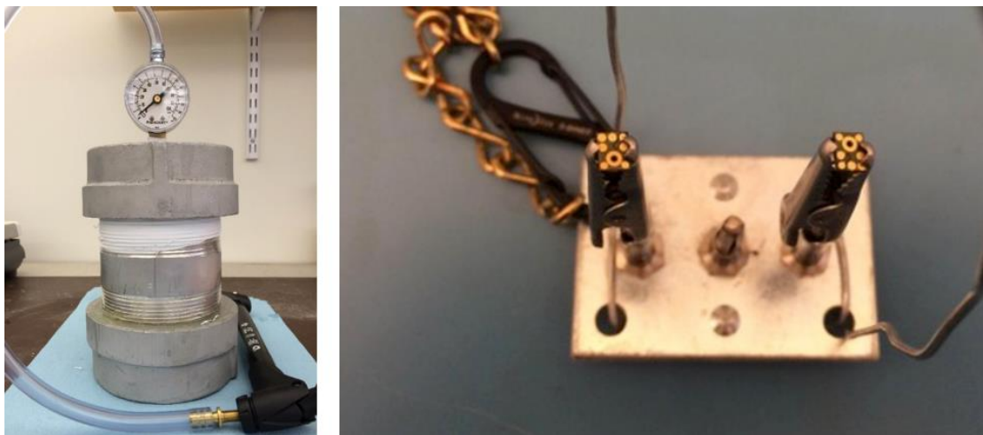
Figure 15: Microphone water-testing apparatus (left) microphones tested with acoustic ports face-up (right)
