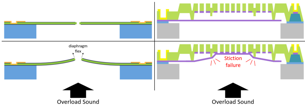
Figure 12: Comparison between acoustic overload behavior of Vesper piezoelectric MEMS microphone (left) and capacitive MEMS microphone (right)
