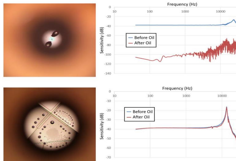
Figure 18: Oil-test image and results on capacitive microphones (upper), Oil-test image and results of Vesper piezoelectric MEMS microphones (lower)
