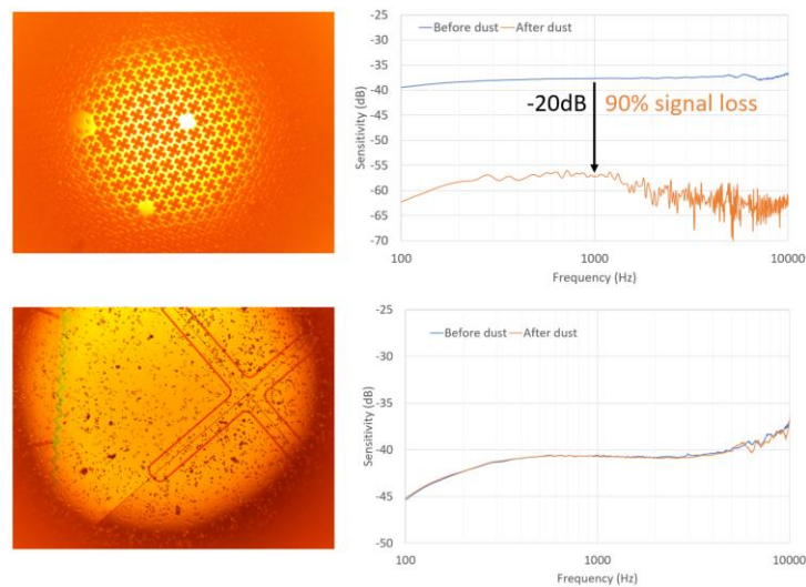
Figure 14: Dust-test image and results of capacitive MEMS microphones (upper), Dust-test image and results of Vesper piezoelectric MEMS microphones (lower)
