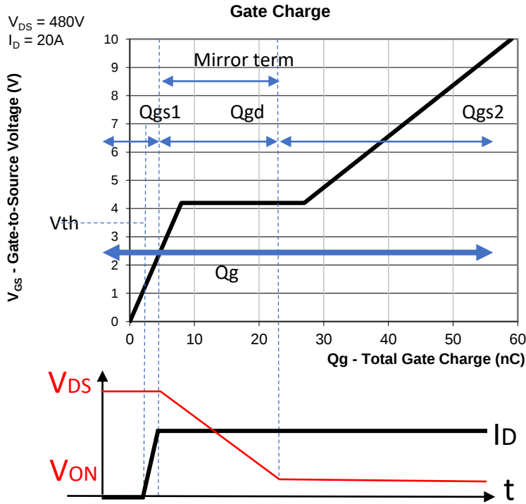
Fig.23 Gate Charge
