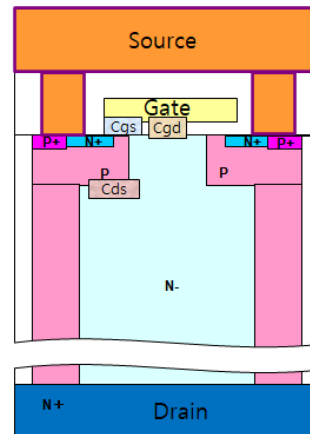
Fig19. Capacitance of the SJMOSFET structure
