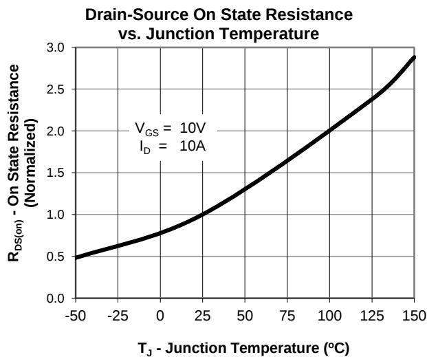
Fig.12 R_{DS(ON)} Vs T_J Junction temperature.
