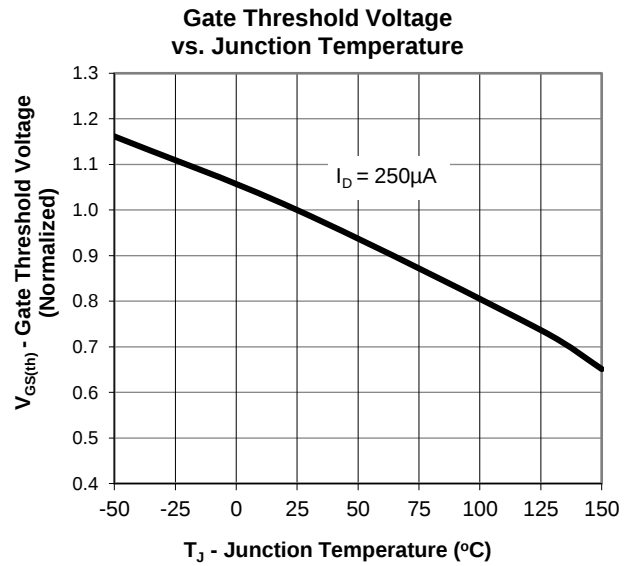
Fig.11 V_{GS(th)} Vs T_J Junction temperature.
