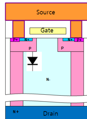
Body Diode
