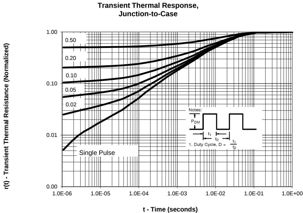
Fig.25 Transient Thermal Resistance r(t) -pulse width time
