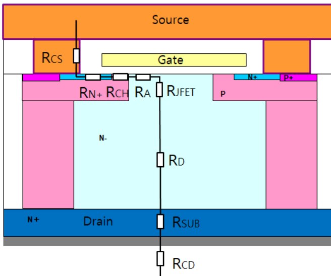
Fig. 9 The Components of ON Resistance
