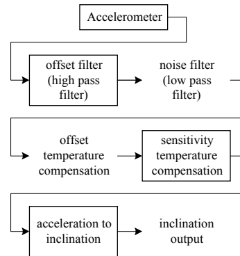
Figure 5: Acceleration to inclination signal processing
