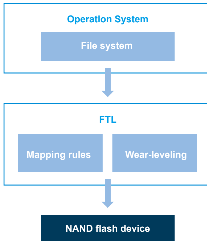
Figure 1 Wear Leveling in the FTL
