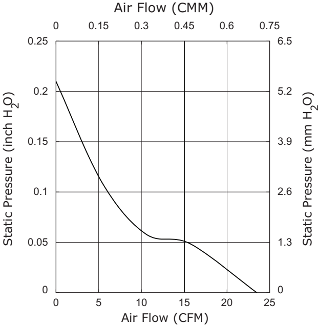
CFM-6025V-145-270
