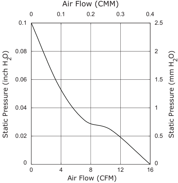
CFM-6025V-231-167
