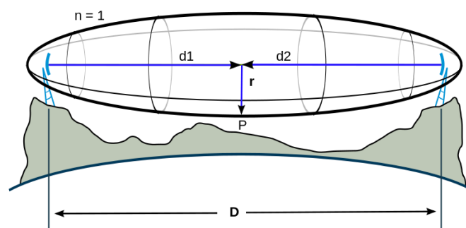
Figure 1. Fresnel Zone.
