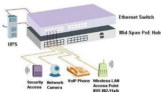
Fig 1A Mid-Span Powered Hub
