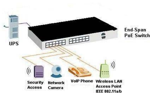
Fig 1B End-Span Powered Switch
