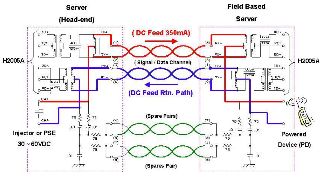
Figure 2 Power-over-Ethernet Example (VoIP application use Pulse H2005A products)
