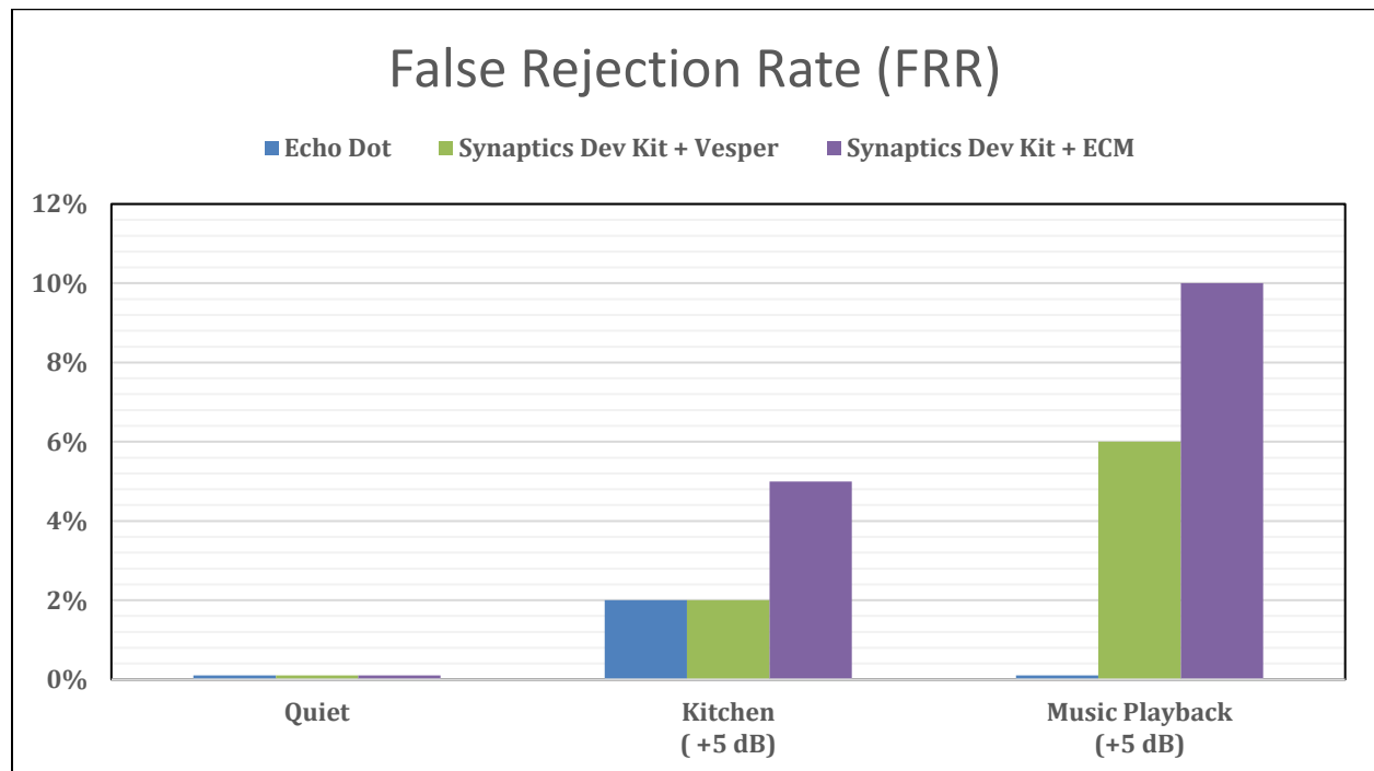
Figure 5: False Rejection Rate (FRR) comparison (lower is better)
