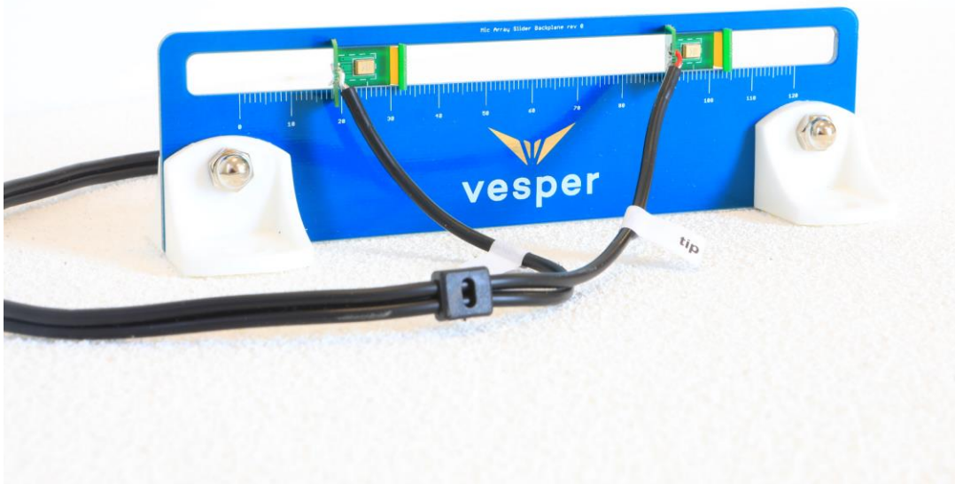
Figure 1: Vesper VM1001 mics on slider – Microphone lids facing on 2 mini-pcbs
