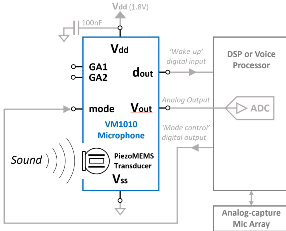
Figure 9: Block diagram of system using VM1010 microphone as 'acoustic watchdog' only
