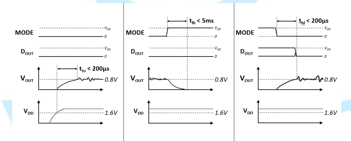
Figure 3: Vout DC and Vdd level timing diagrams showing turn-on time (left), transition time into Wake-on-Sound mode (center) & Full-Power mode (right)
