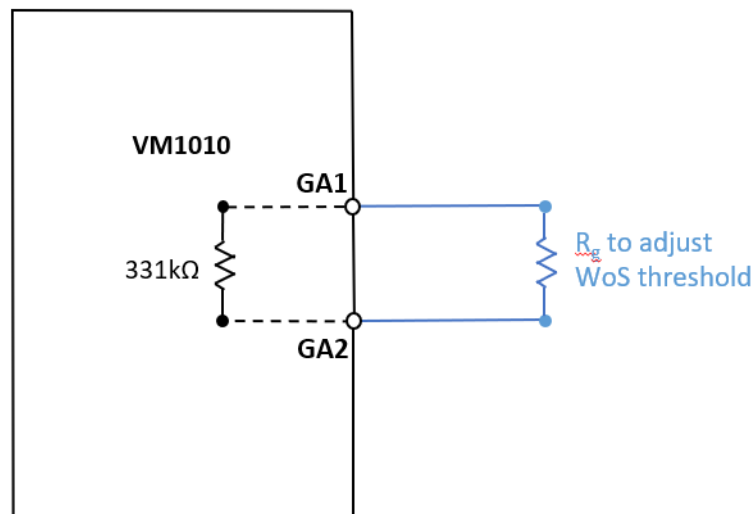
Figure 6: Fixed adjusted WoS threshold, implemented with external resistor ( R_g ) between GA1 and GA2 pins
