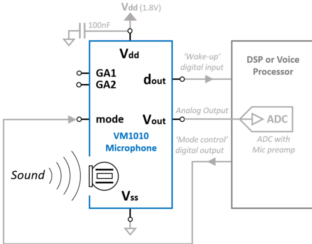
Figure 8: Block diagram of full-featured system built around VM1010 microphone
