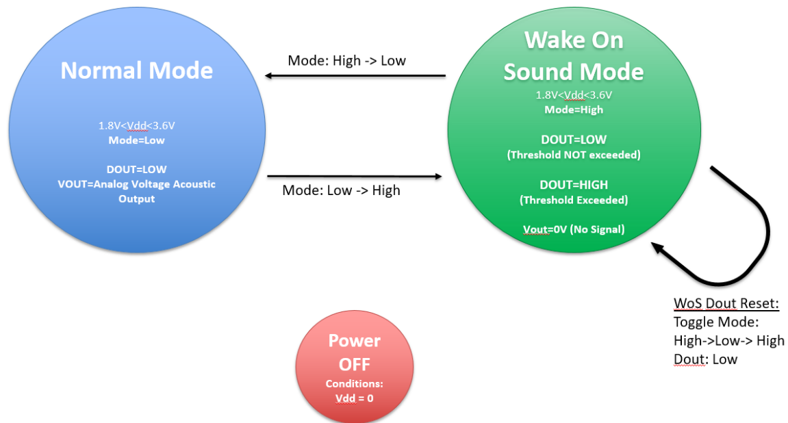
Figure 2: State diagram of VM1010 modes and relevant transitions
