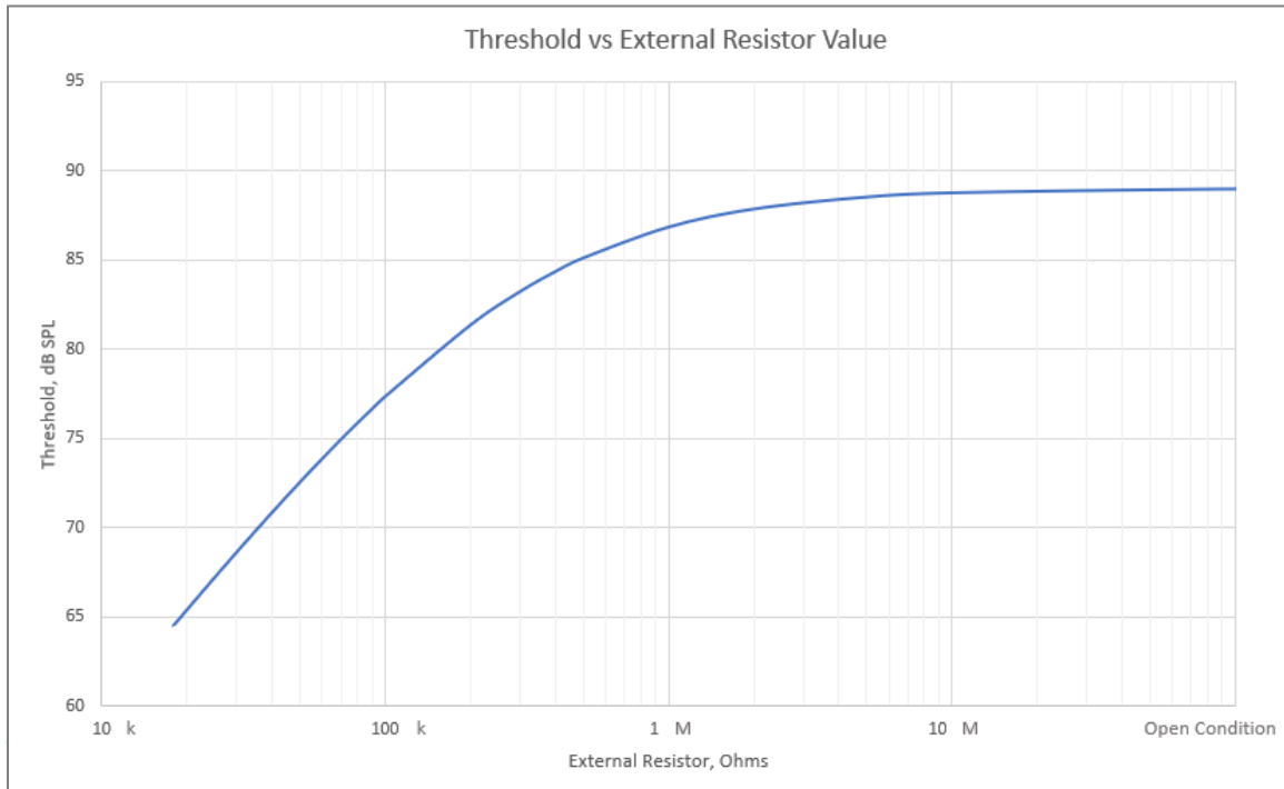
Figure 7: Graph of WoS threshold versus external gain resistor ( R_g )
