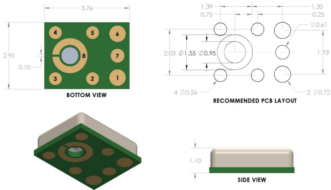
Figure 1: Mechanical drawing of VM1010 Microphone
