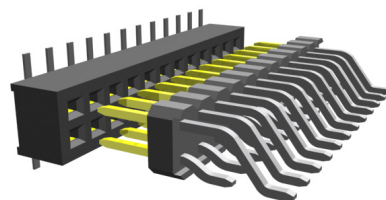
SMT male & female Header B-t-B combination
