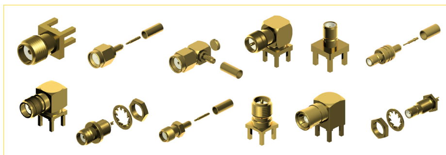
SMA / SMA Reverse / SMB Types
