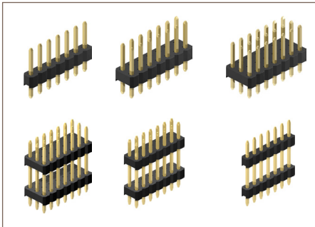
THT Pin Header Board Spacer straight
