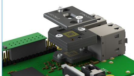
Socket for end customer PCB (Test socket for PCB not intended to accept socket)
