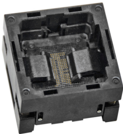
Burn in socket
