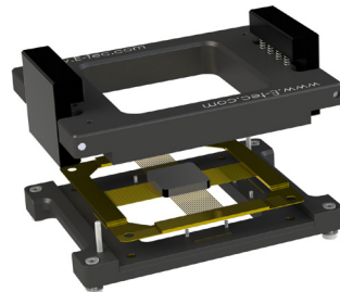
Open Top socket
