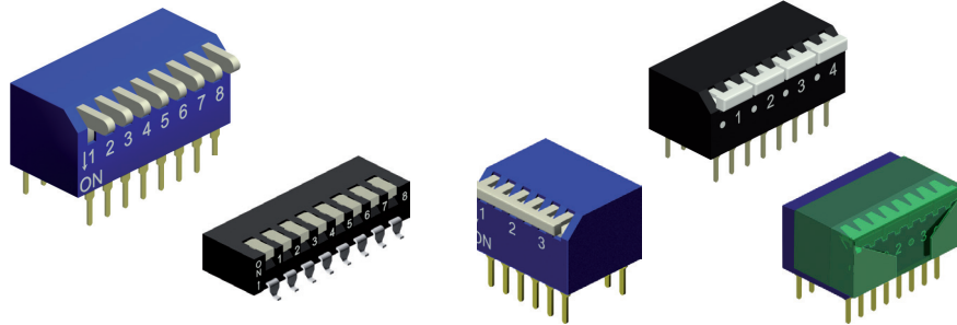
THT & SMT Piano Switches
