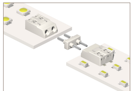
LED Connectors
