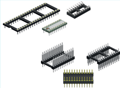
DIL-Sockets/Spacer/Adapter (THT - SMT - LowProfile - Capacitors)
