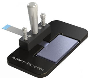
Flat Flex Cable, Display & Test Unit
