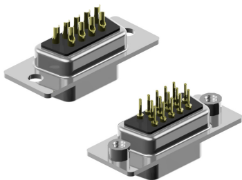
Solder Cup & Solder Tail
