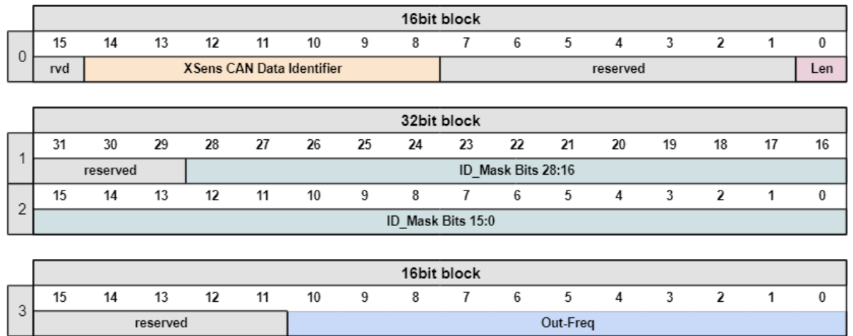
Figure 4 SetCanOutputConfig structure
