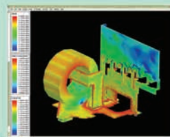
EMI Field Simulation
