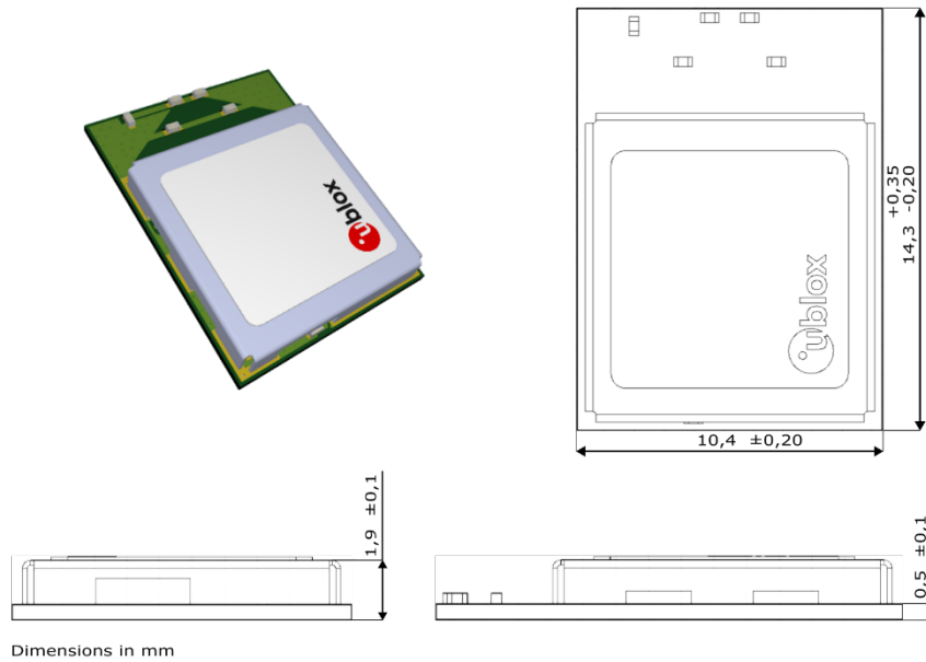
Figure 6: NORA-W256AWS dimensions
