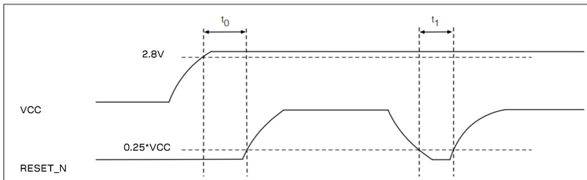
Figure 4: Module power-up and reset timing
