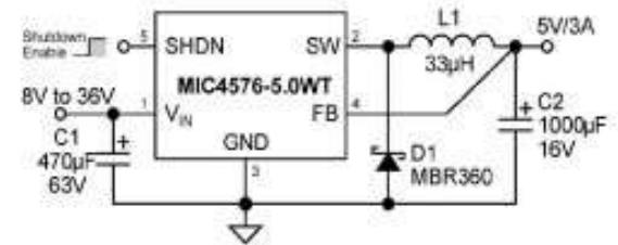
Fixed Regulator
