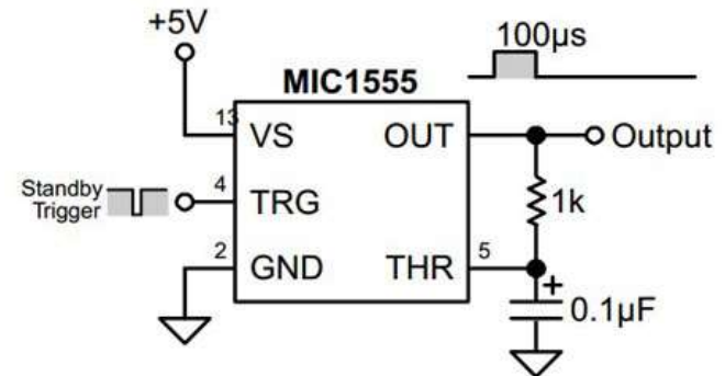
Monostable (One-Shot)
