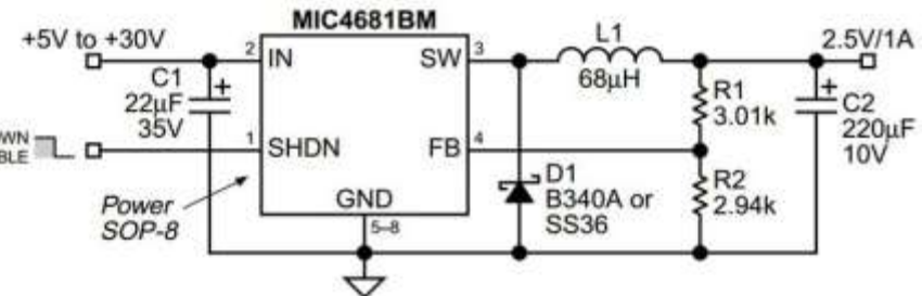
Adjustable Regulator Circuit
