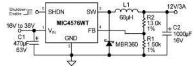
Adjustable Regulator
